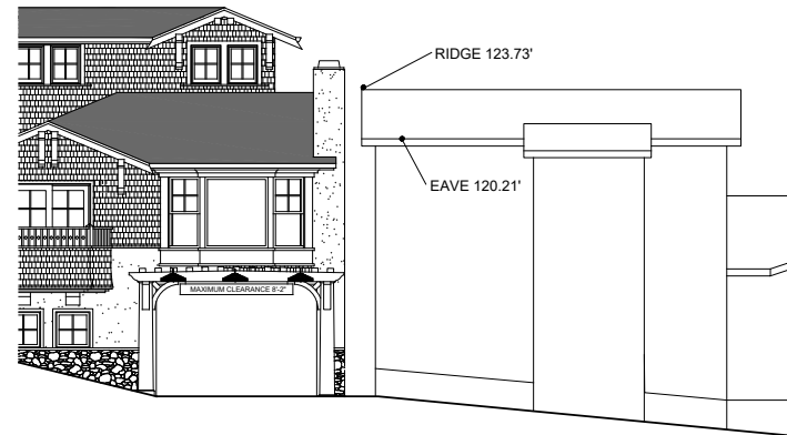
FIFTH AVENUE STREETSCAPE ENLARGED ELEVATION SCALE: 1/4"=1'-0"
